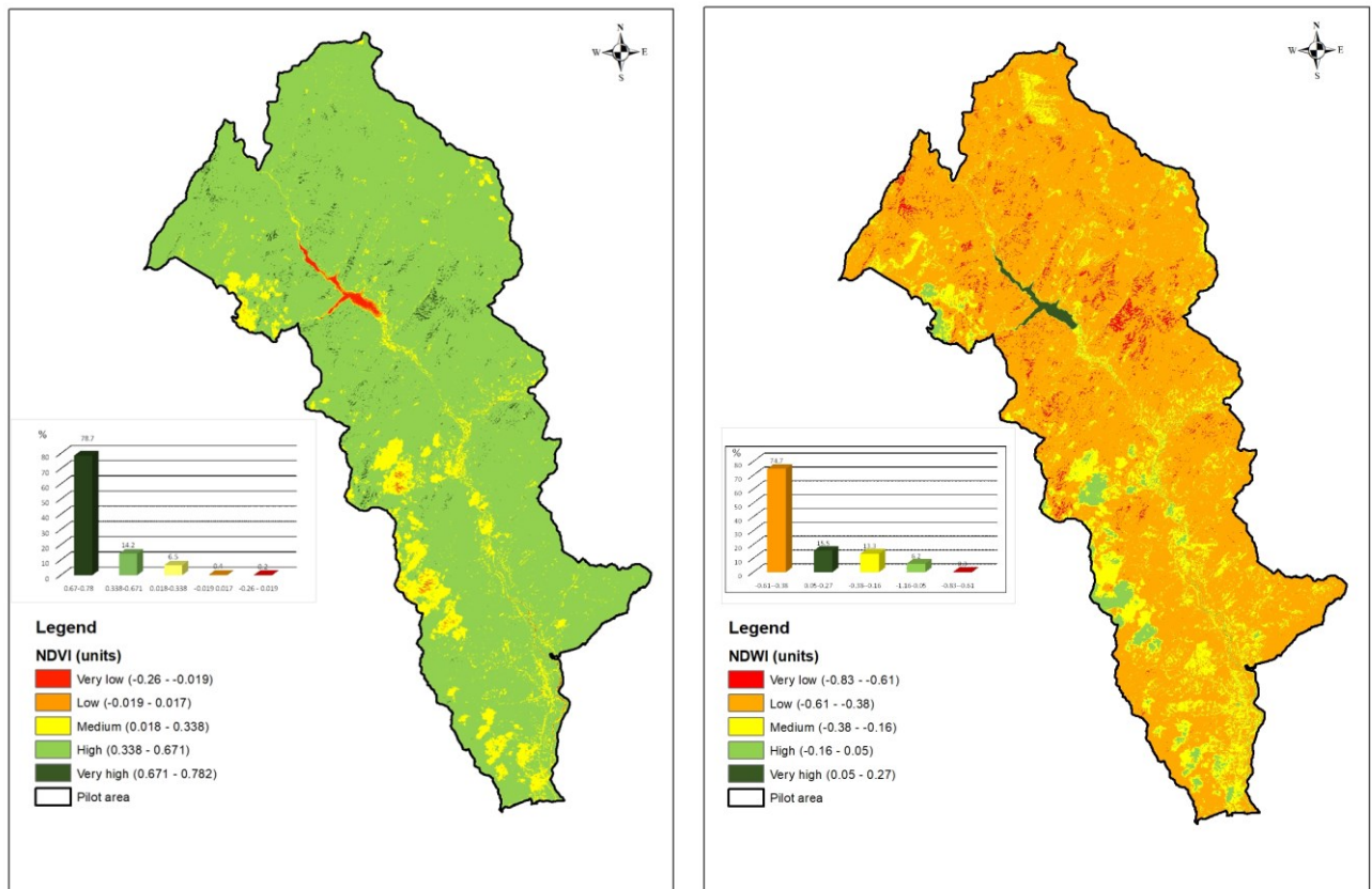
Fig.4. NDVI and NDWI maps of the Romanian pilot area
