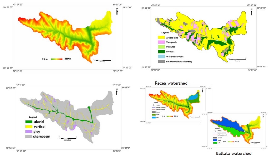
Figure 1. The a) DEM, b) the land-use, c) the soils and d) the two studied watersheds.
