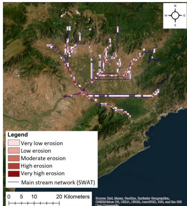
Figure 3. The GIS Stream Bank Erosion Index for the Aggitis Basin in the main SWAT’s stream network. Five classes represent different rates of stream bank erosion: very low, low, moderate, high and very high.
