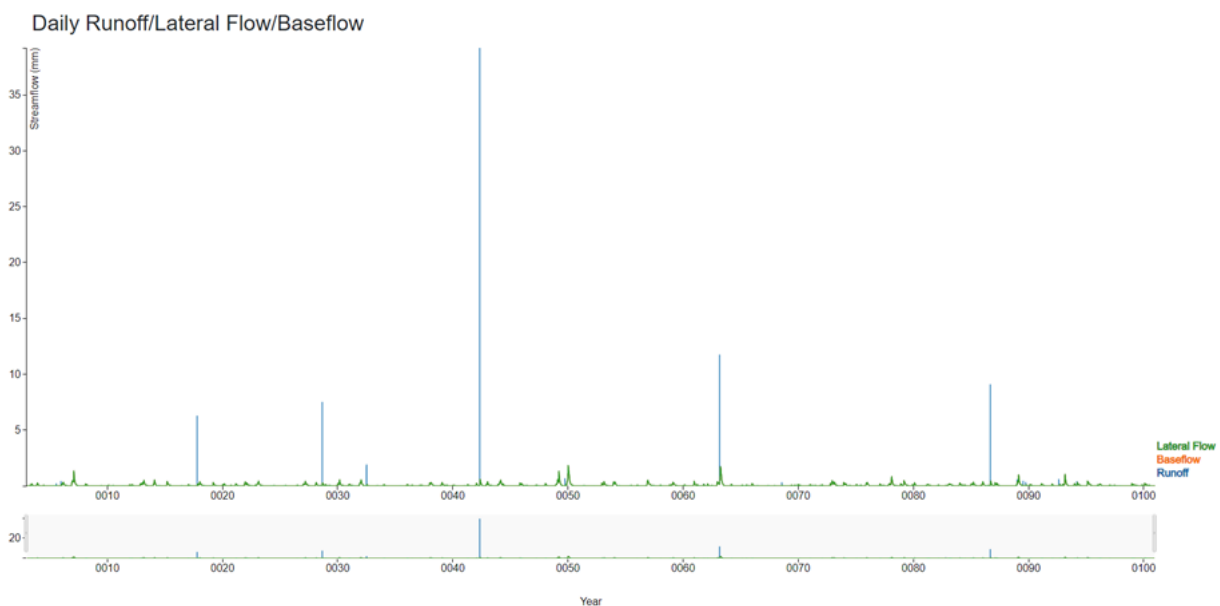
Figure 3. The daily runoff/lateral flow/baseflow.
