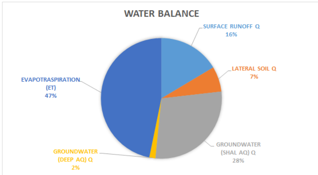
Figure 4. The simulated average water balance of the Aggitis Basin.
