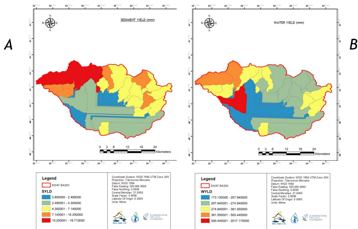
Figure 6. The simulated average a) water yield and b) sediment yield per sub-watershed.
