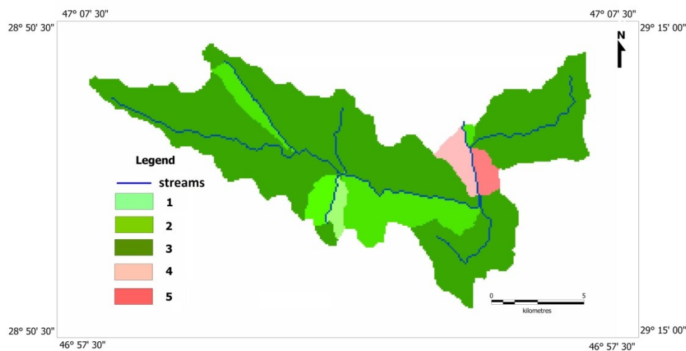
Figure 3. Map of GeoWEPP offsite simulation of annual sediments distribution in the Baltata River watershed for the period 1990-2010. The sediment yield (ton) is classified as: 1) 0 \leq \text{Yield} < \frac{1}{4} ; 2) \frac{1}{4} \leq \text{Yield} < \frac{1}{2} ; 3) \frac{1}{2} \leq \text{Yield} < 1 ; 4) 1.0 \leq \text{Yield} < 2.0 ; 5) 2.0 \leq \text{Yield} < 3.0 .
