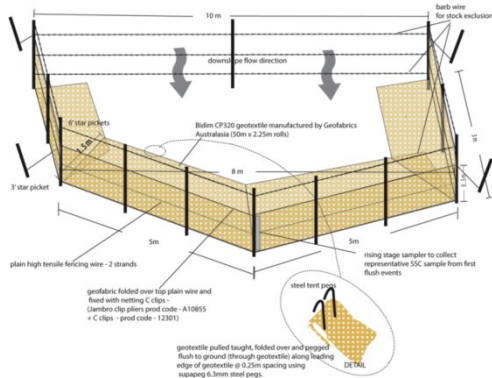
Fig.1. Sketch of a type alluvial Gerlach trap
