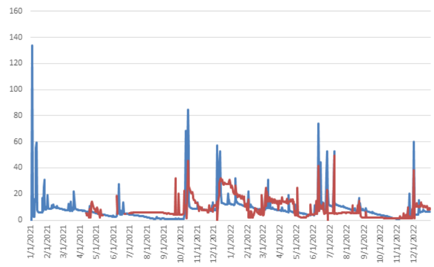
Figure 3. The simulated (blue line) and the recorded water discharge by the installed telemetric hydrologic station in Simvoli Bridge (Aggitis River).
