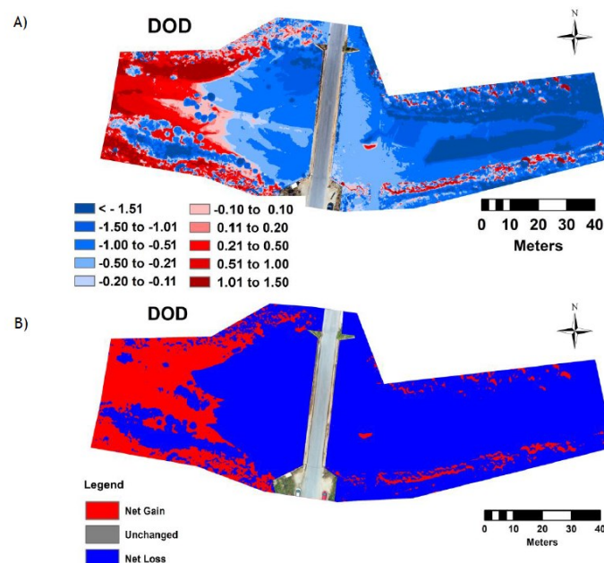
Figure 2. The DoD resulted from the comparison of the images between the dates 14 September 2022 (a) and 28 October 2022 (b). The colorized scale represents the different elevation categories (in meters). The 3 classes: (red) gained material, (grey) unchanged elevation and (blue) loss material.
