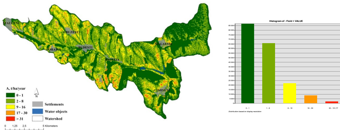
Figure 2. Mean annual soil loss
