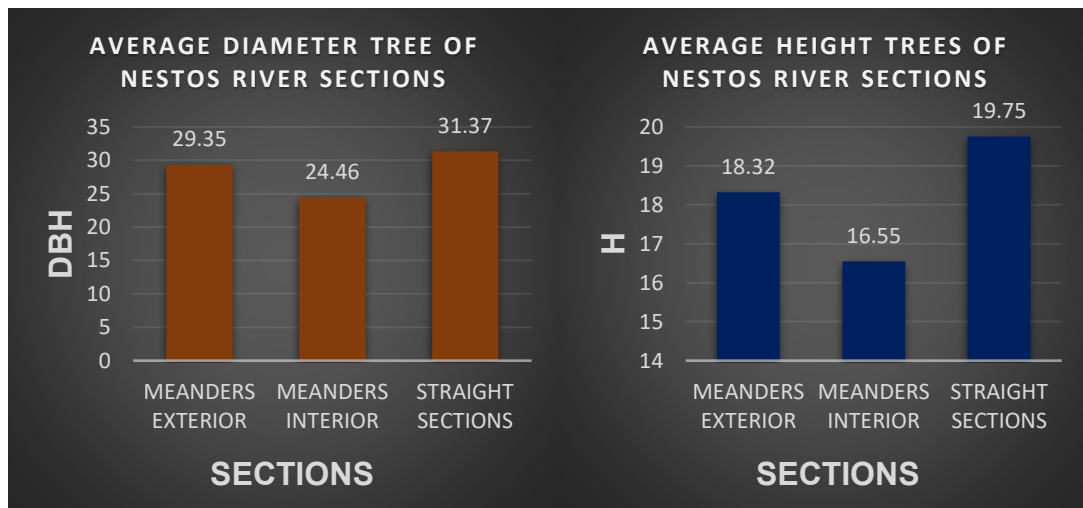
Figure 4. The average diameter and average height of woody vegetation at each geomorphological location in Nestos river.
