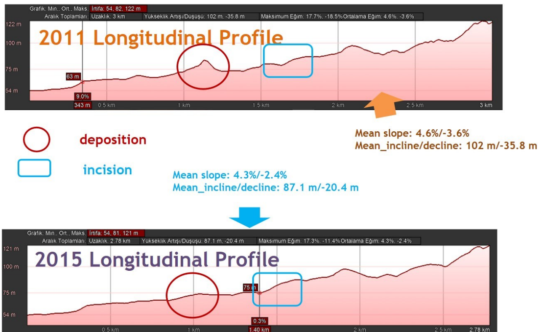
Figure 5. The longitudinal profiles dated in 2011 and 2015 showed that the average slope was 4.6% and 4.3% respectively. The mean incline was 102 m for 2011 and 87.1 m for 2015.
