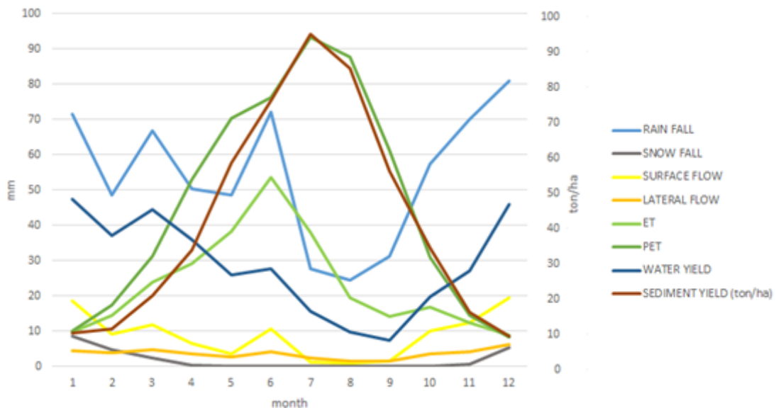
Figure 5. The simulated average monthly values of hydrologic phases of the Aggitis Basin.
