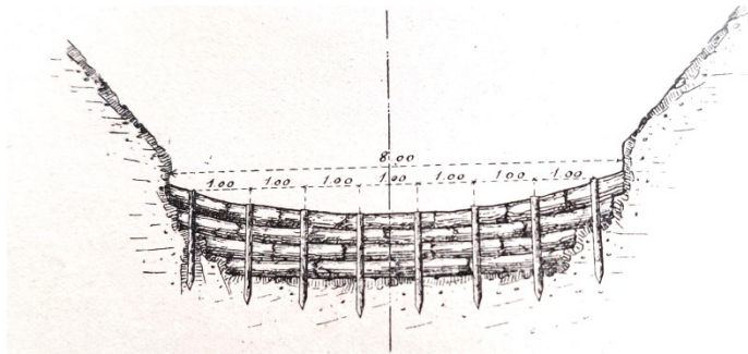
Figure 3. Wooden check dam on torrents in French (Source: Thiery [8])
