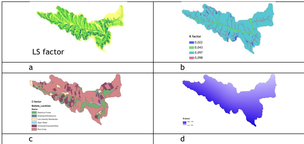
Figure 1. Baltata river basin, spatial distribution for LS factor, dimensionless (a), K-factor, (\text{tons} \cdot \text{ha} \cdot \text{h}) / (7.59 \cdot \text{ha} \cdot \text{MJ} \cdot \text{mm}) (b), C-factor, dimensionless (c), and R-factor, (\text{Mj} \cdot \text{mm}) / (\text{ha} \cdot \text{h} \cdot \text{yr}) (d)
