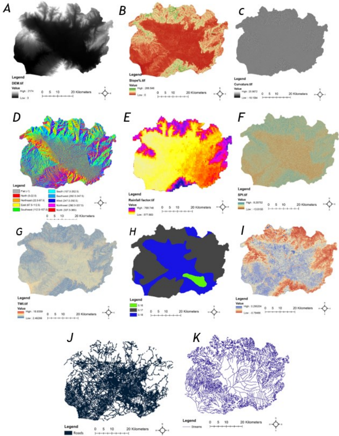
Figure 1. The a) DEM, b) slope (%), c) curvature, d) aspect, e) rainfall erosivity index, f) stream power index, g) topographic wetness index, h) soil erodibility index, i) normalized difference vegetation index, j) infrastructure index and k) water yield index for the Aggitis Basin.
