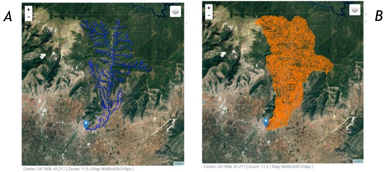
Figure 1. a) the stream network and b) the sub-watersheds of Kallifitos watershed.
